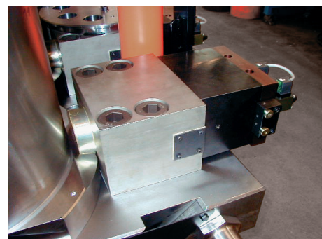
Wedge clamps on a forging press
