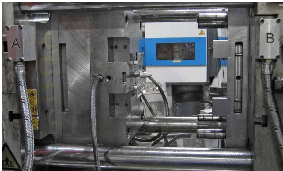
Magnetic clamping system integrated in a die casting machine
